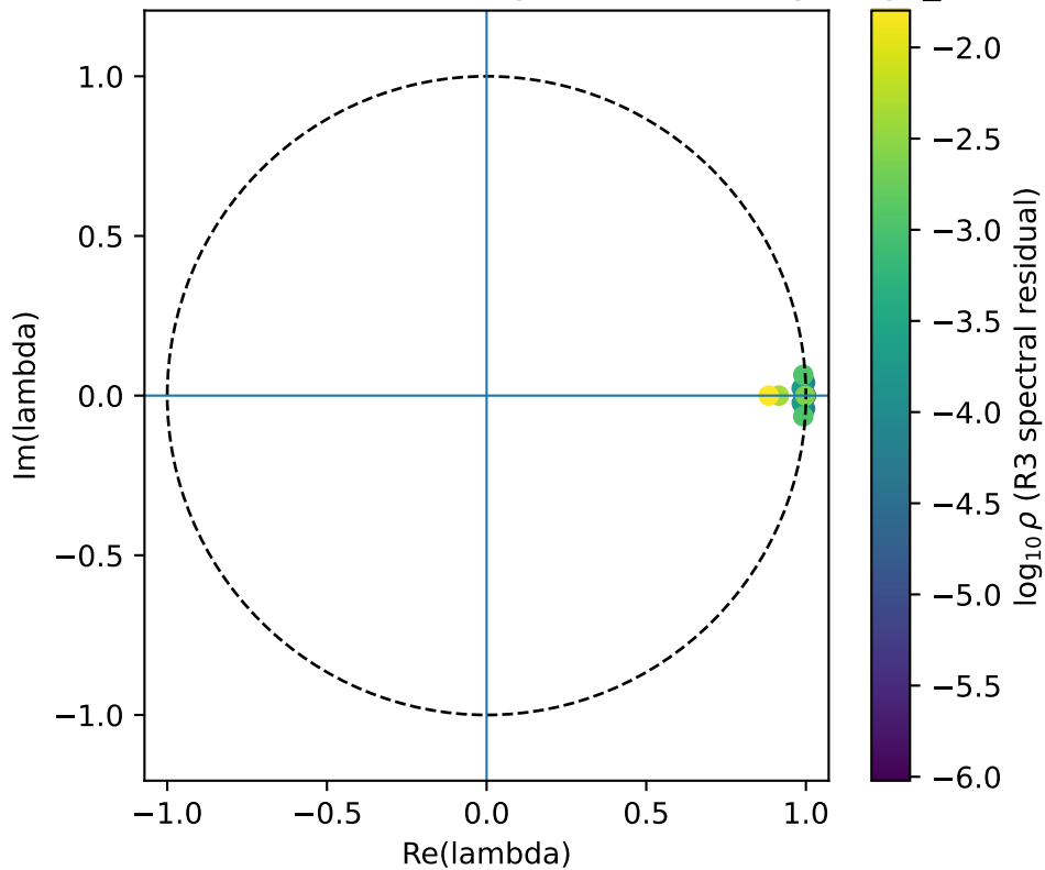
R3 residual-verified KAHKM spectrum: duffing, ridge_ls
