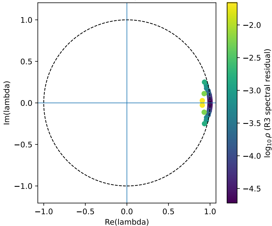
R3 residual-verified KAHKM spectrum: vanderpol, nlms
