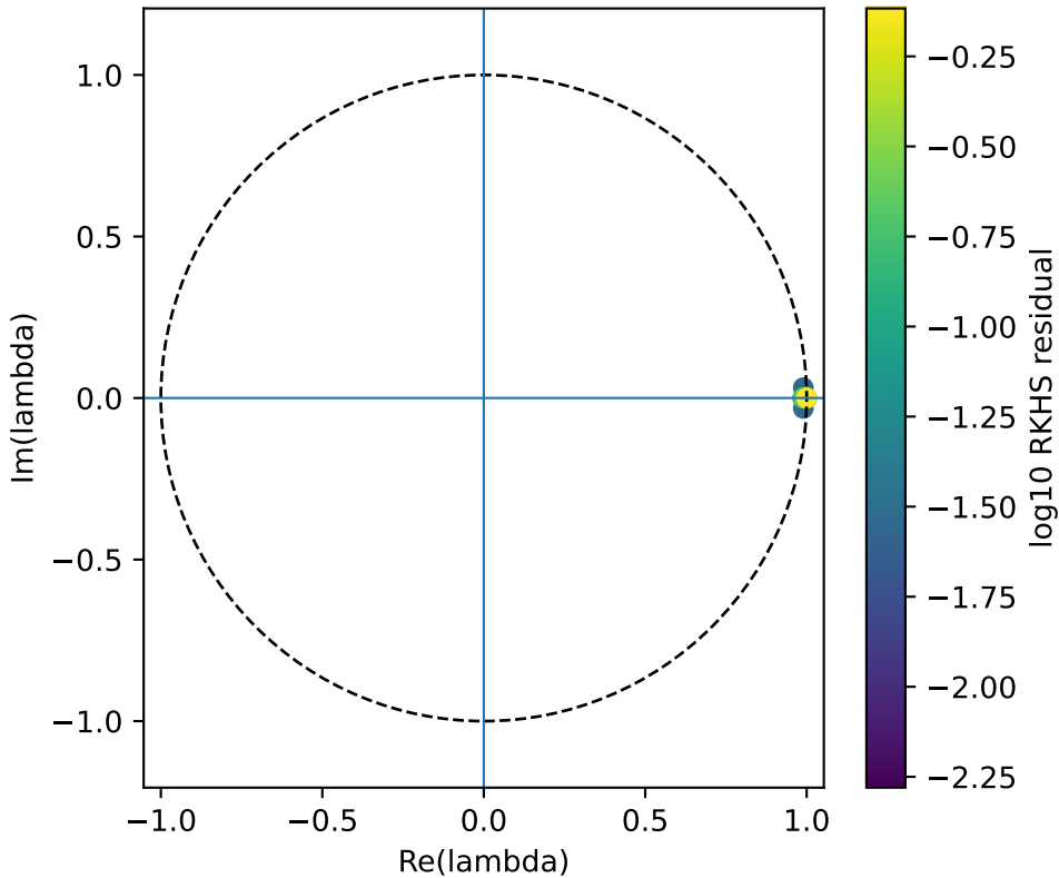
Residual-verified KAHKM spectrum: duffing, nlms
