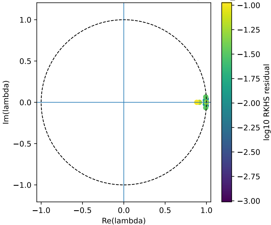
Residual-verified KAHKM spectrum: duffing, ridge_ls
