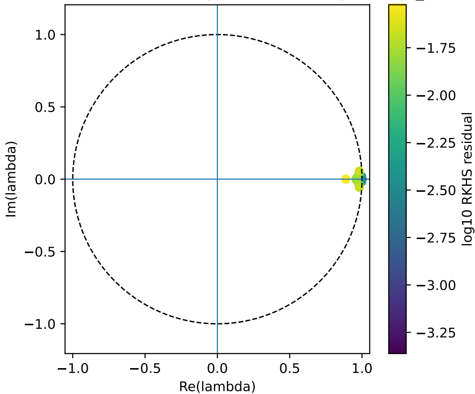
Residual-verified KAHKM spectrum: vanderpol, ridge_ls
