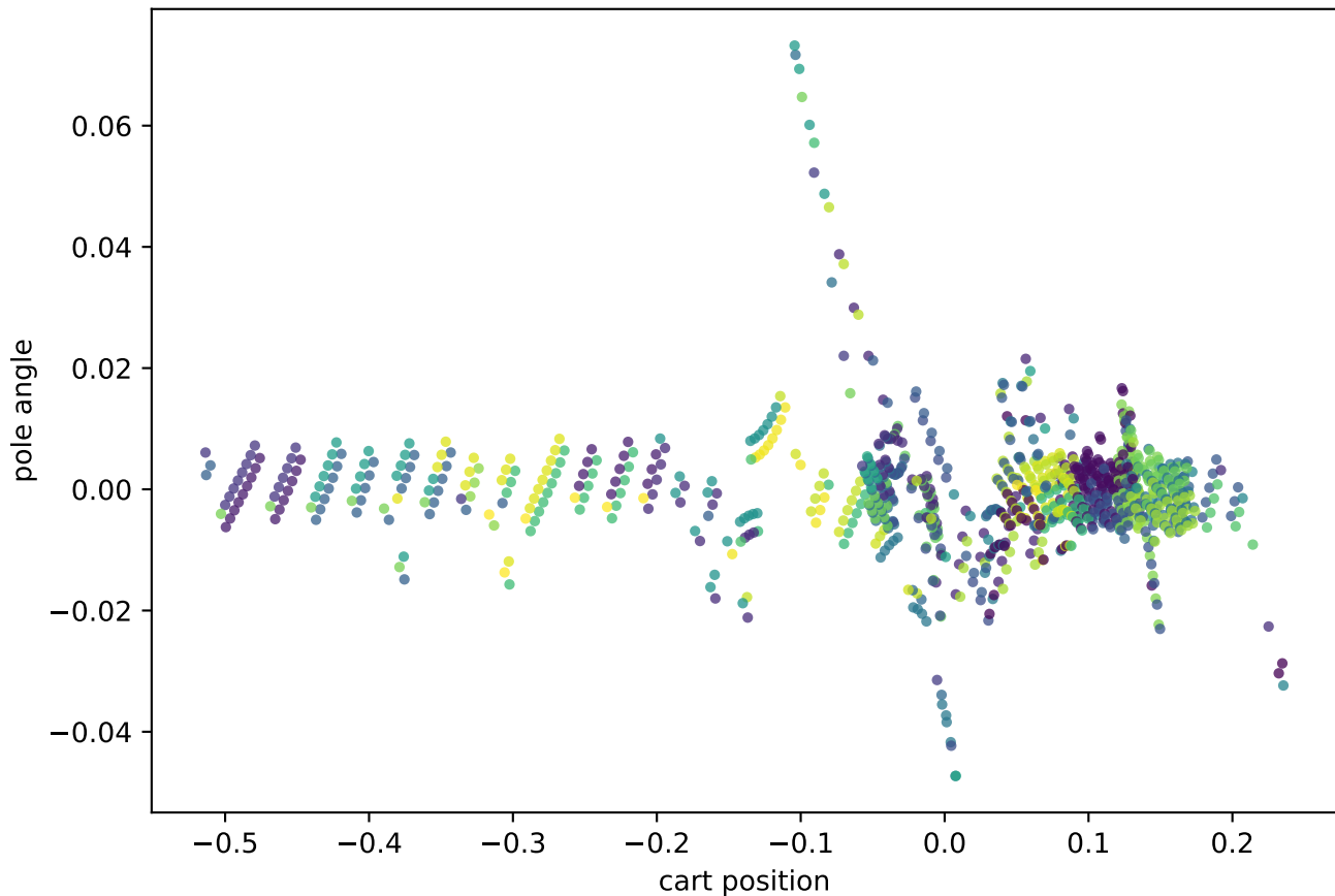
CartPole-v1: dominant KAHKM regime
