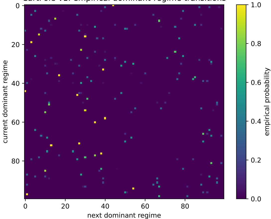
CartPole-v1: empirical dominant-regime transitions
