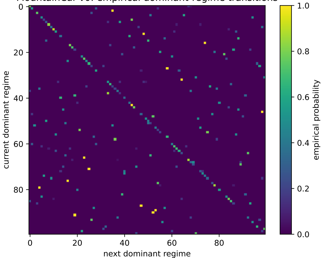
MountainCar-v0: empirical dominant-regime transitions
