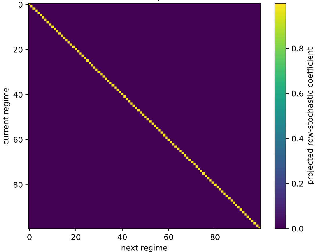
MountainCar-v0: learned interpretable transition matrix
