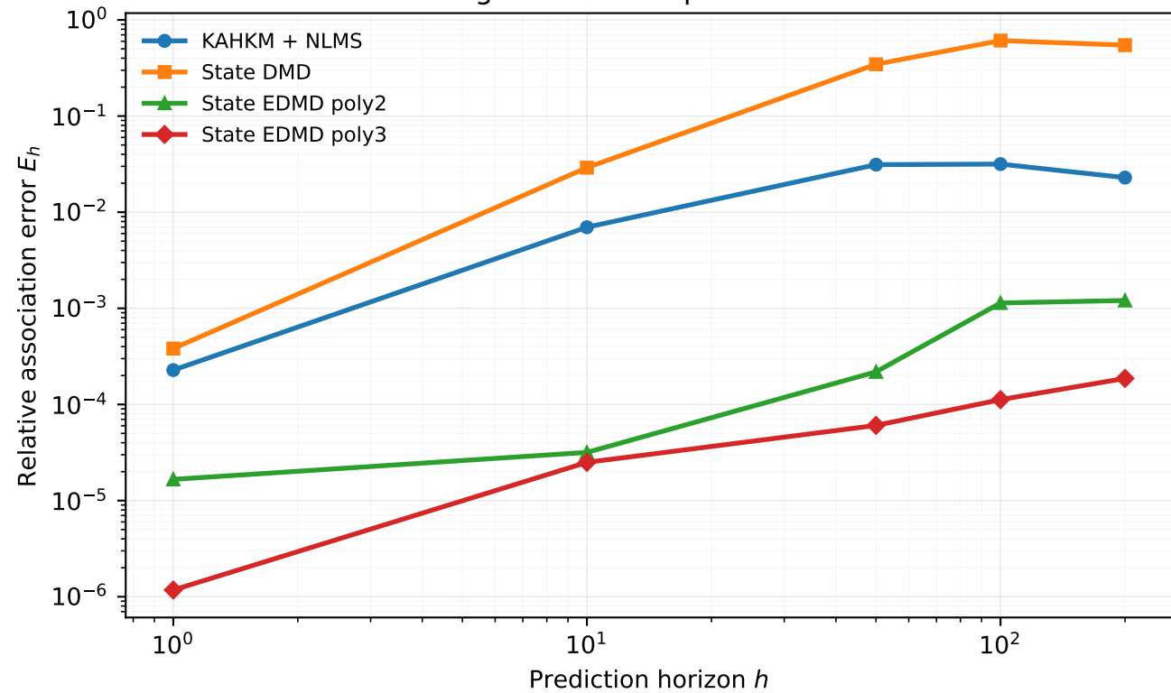
Duffing external Koopman baselines
