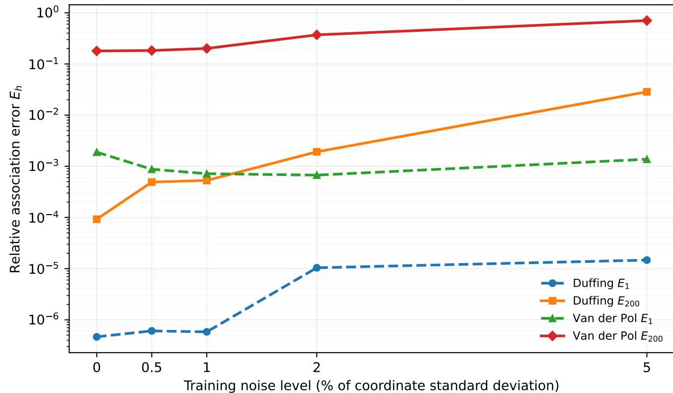
Default noise robustness diagnostic
