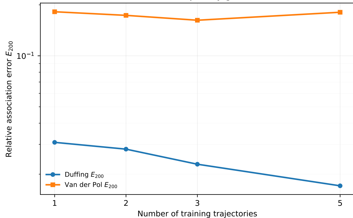
Default unseen-trajectory generalization
