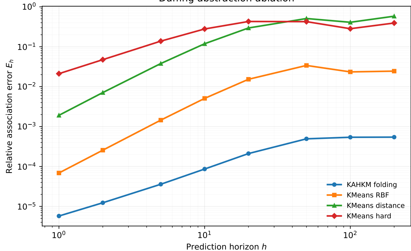
Duffing abstraction ablation
