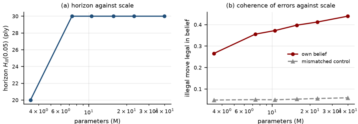
Figure 5: (a) The horizon against model size. (b) Belief consistency and its matched control against model size. The question is whether the mechanism is a property of small models or survives scale.
