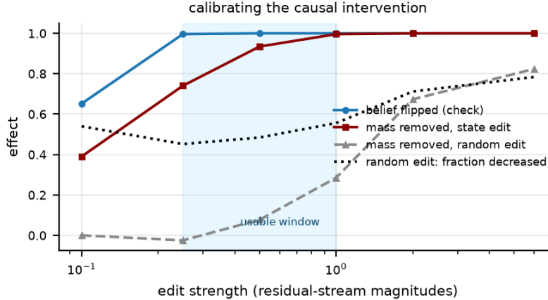
Figure 6: Choosing the edit strength. Too small and the belief does not flip; too large and a norm-matched random direction also destroys the output distribution, so any effect there is damage rather than belief. We report inside the shaded window.
