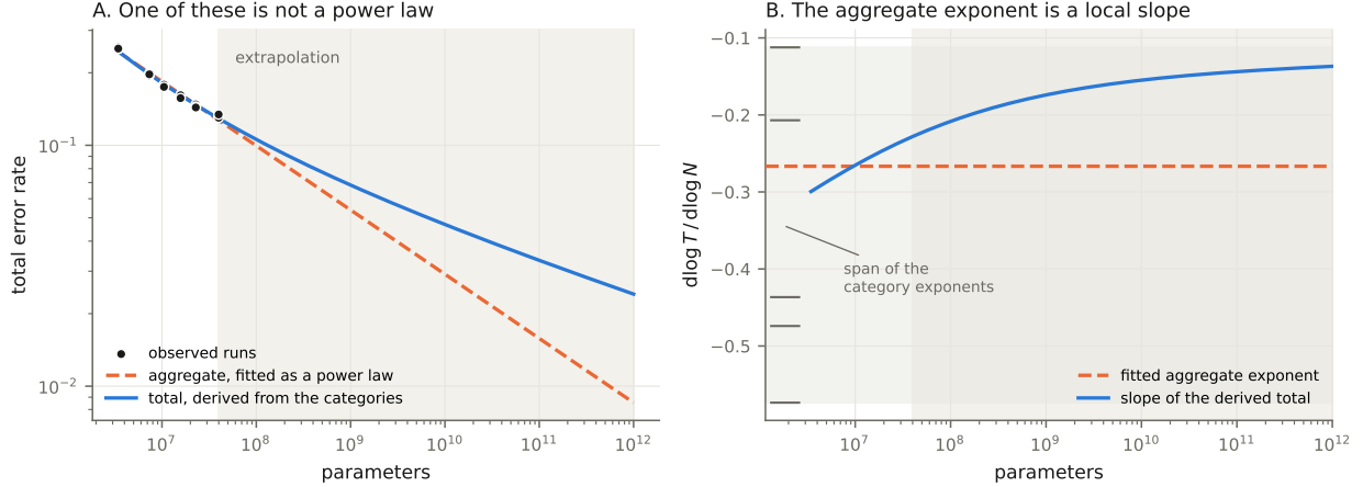
Figure 1: The two objects the paper says cannot both be reported. Panel A: on log-log axes a power law is a straight line, so the fitted aggregate is straight by construction while the derived total, the sum of the same category curves, bends. Both agree with the observed runs, which is why nothing in range distinguishes them; the gap opens only in the shaded extrapolation region where the forecast was actually read. Panel B: the same fact as a slope. A power law contributes one exponent everywhere, shown flat, while the derived total’s slope drifts across a substantial part of the band spanned by the category exponents, drawn as rules at the left. The aggregate exponent is the height of the dashed line; it is a local property of the fitted range, not of the system.
