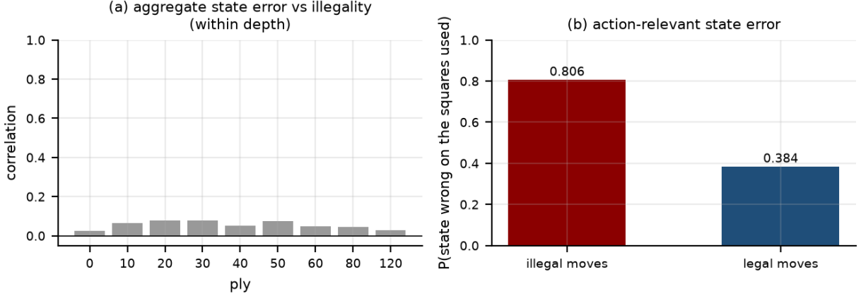
Figure 3: (a) Within a fixed depth, the correlation between the number of misremembered squares and playing an illegal move is close to zero. (b) The same representation, scored only on the squares the move actually uses, separates illegal from legal moves sharply.
