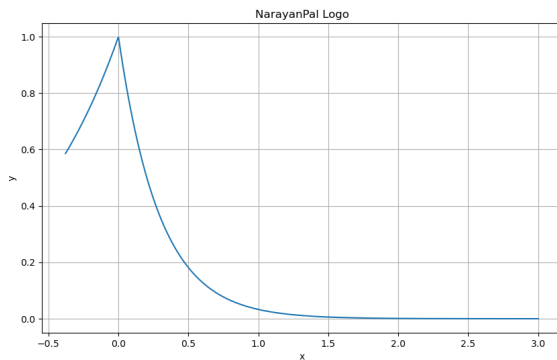
Fig. 3: Truncated Function f(t) for a = \sqrt{2} + 2 and b = \sqrt{2}
