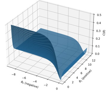
Fig. 4: C(\theta) for a = \sqrt{2} + 2 and b = \sqrt{2}
