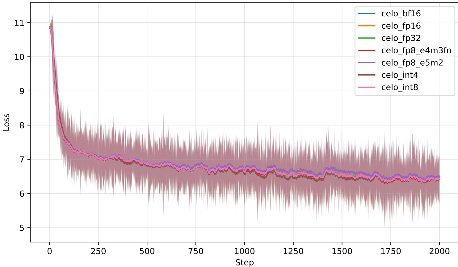
TransformerLM_LM1B: CeLO quant sweep (EMA-smoothed mean \pm std)
