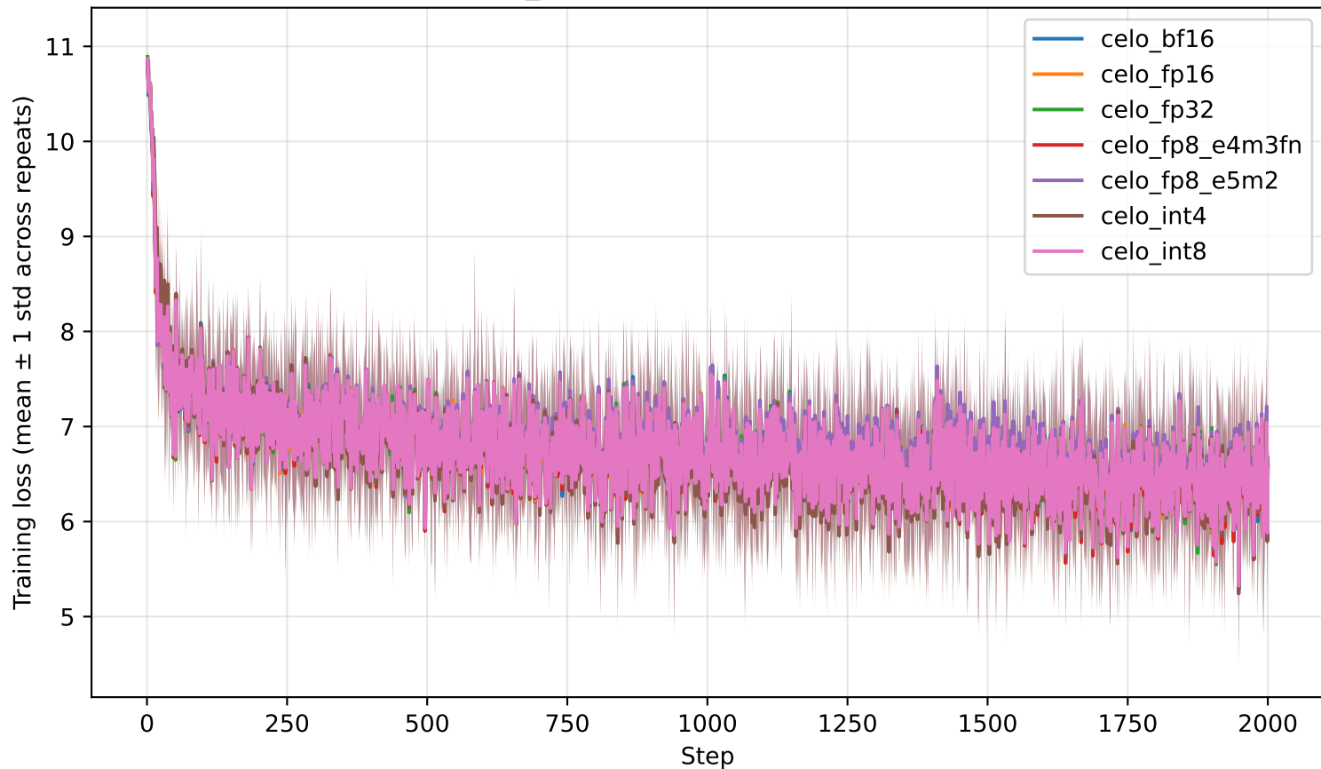
TransformerLM_LM1B: CeLO quant sweep (mean \pm std)
