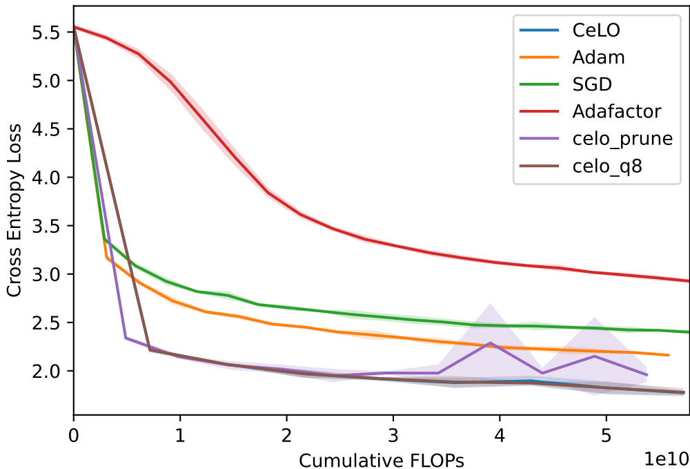
Optimizers Training Loss vs. FLOPs
