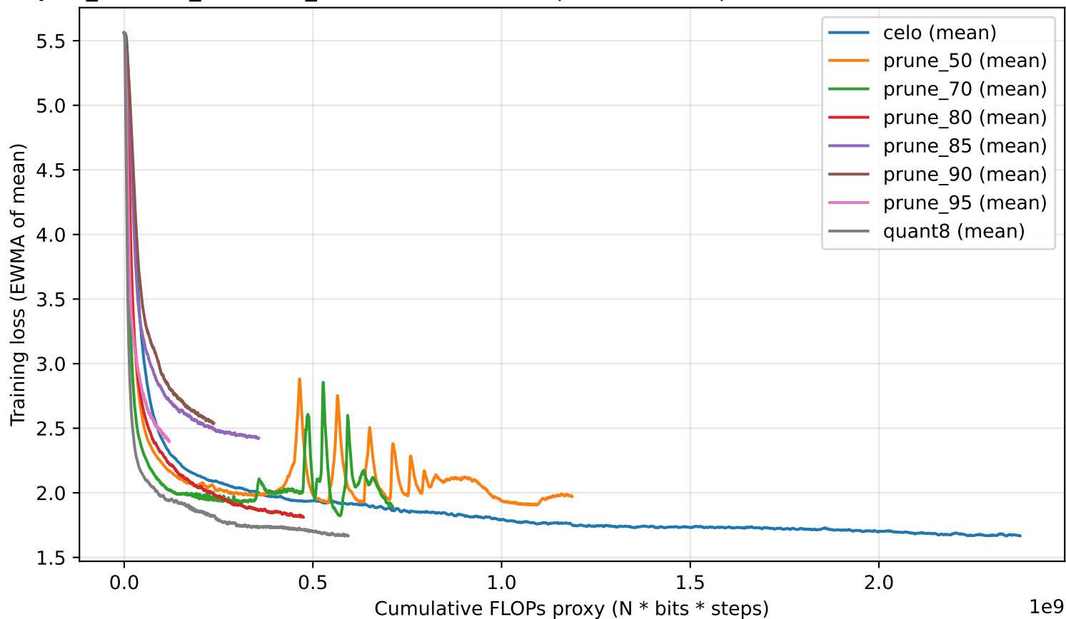
11bytes_Patch32_LSTM128_Embed64: CeLO compression sweep (mean \pm std vs FLOPs over 1 s
