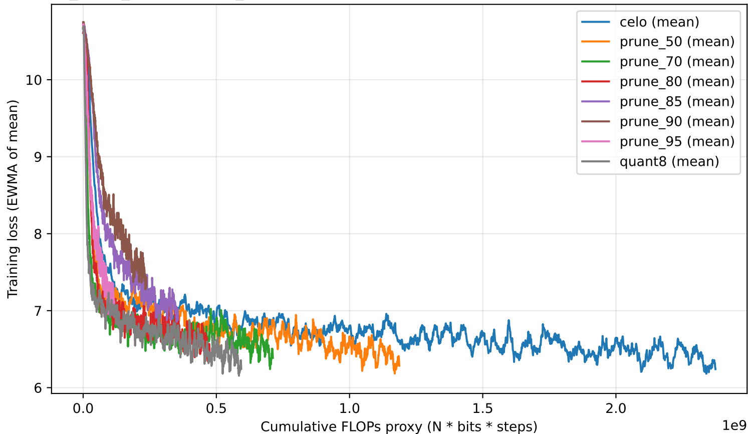
formerLM_LM1B_MultiRuntime_0: CeLO compression sweep (mean \pm std vs FLOPs over 1 seeds,
