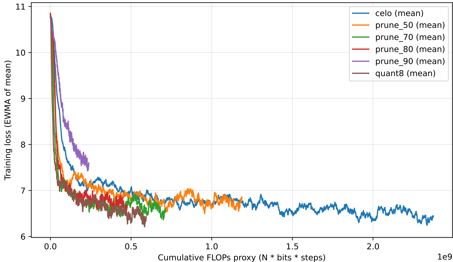
CeLO compression sweep: mean \pm std vs FLOPs over 1 seeds (span=50)
