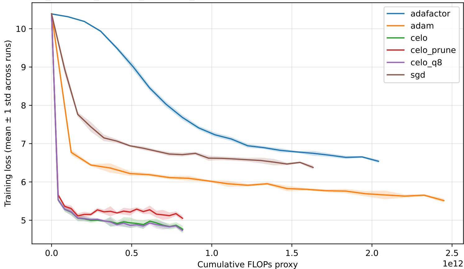
RNNLM_lm1b32k_Patch32_LSTM256_Embed128: Training Loss vs FLOPs (mean \pm std over runs)
