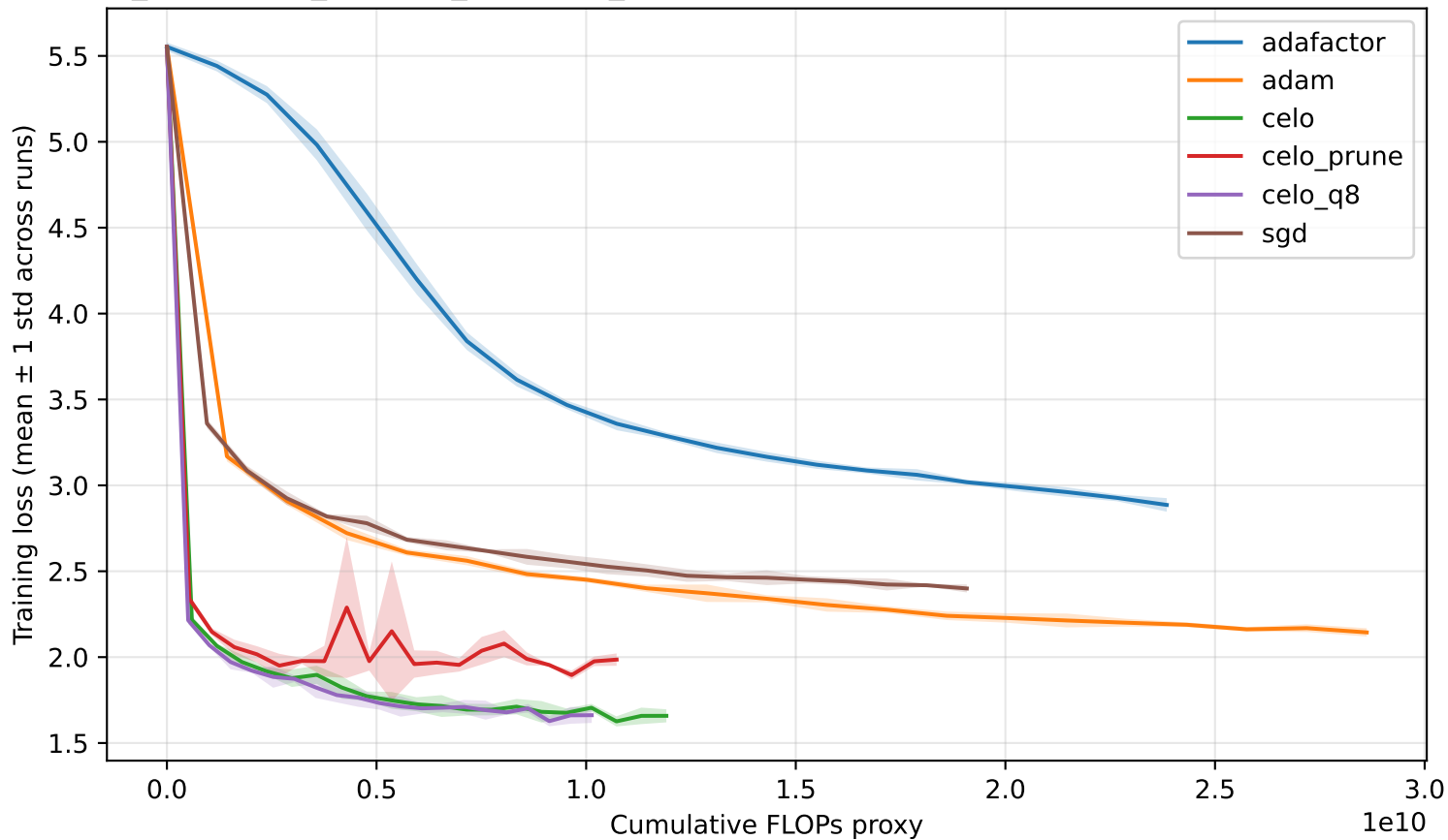
RNNLM_Im1bbytes_Patch32_LSTM128_Embed64: Training Loss vs FLOPs (mean \pm std over runs)
