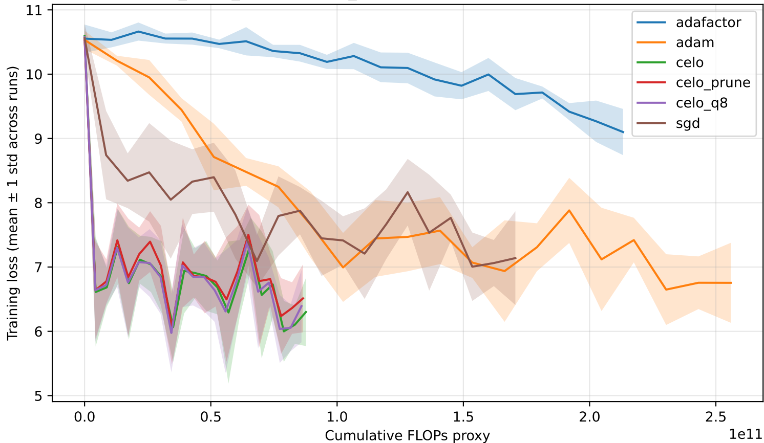
TransformerLM_LM1B_MultiRuntime_0: Training Loss vs FLOPs (mean \pm std over runs)
