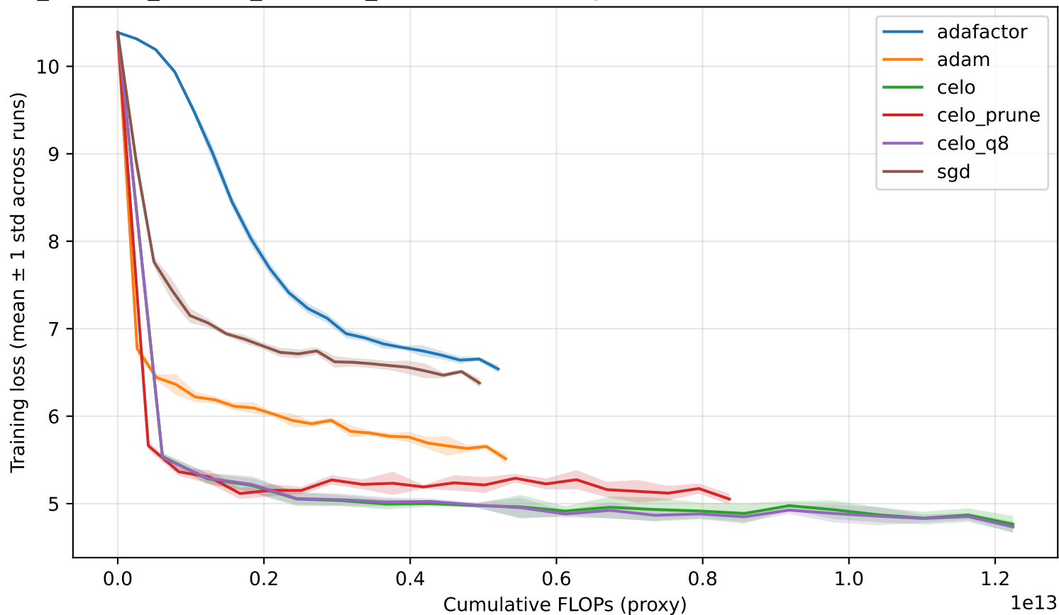
NLM_lm1b32k_Patch32_LSTM256_Embed128: Training Loss vs cumulative FLOPs (mean \pm std over runs)
