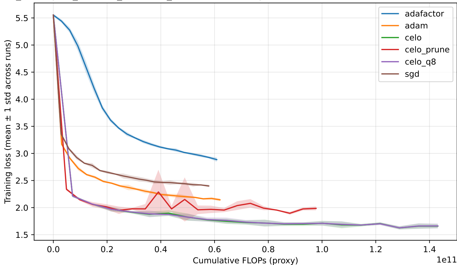
NLM_lm1bbytes_Patch32_LSTM128_Embed64: Training Loss vs cumulative FLOPs (mean \pm std o
