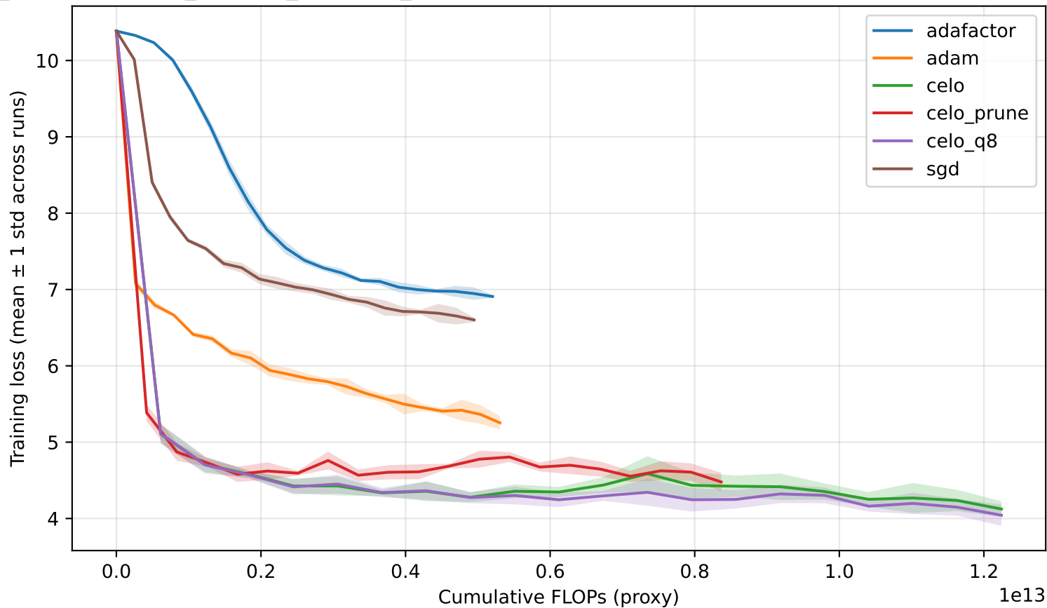
1_wikipediaen32k_Patch32_LSTM256_Embed128: Training Loss vs cumulative FLOPs (mean \pm std across runs)
