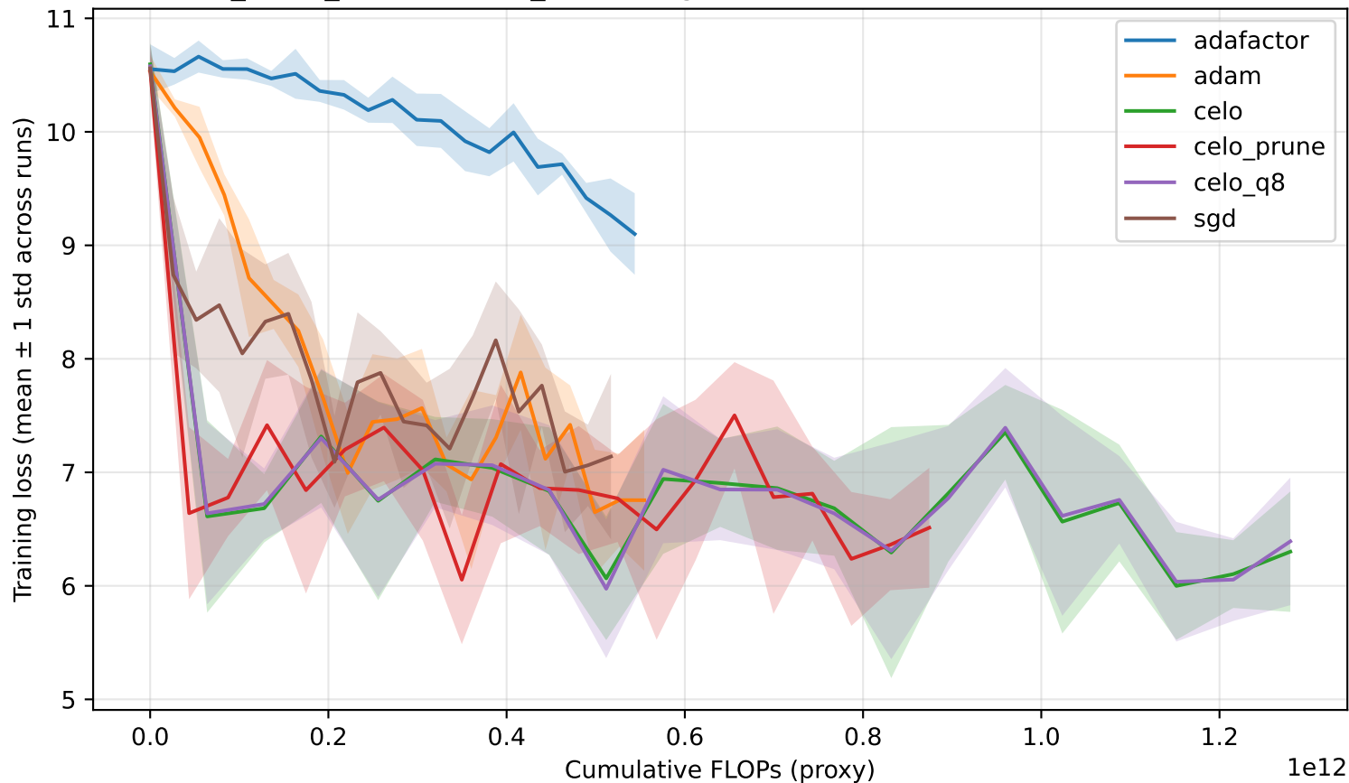
TransformerLM_LM1B_MultiRuntime_0: Training Loss vs cumulative FLOPs (mean \pm std over runs)
