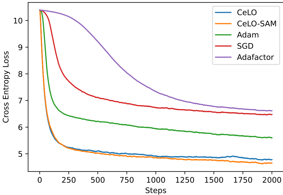
Optimizers Training Losses vs. Step
