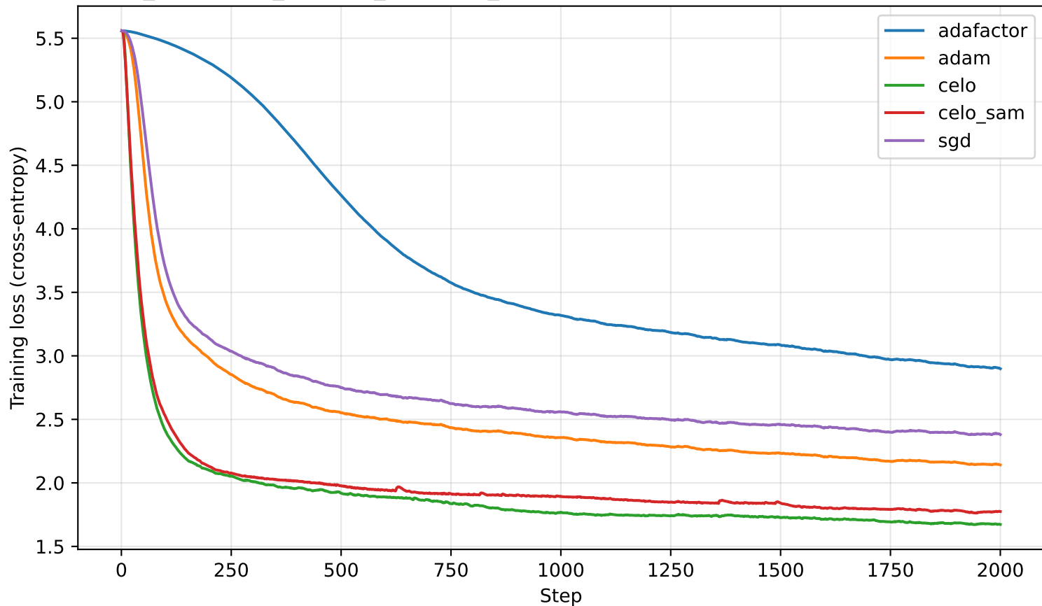
RNNLM_Im1bbytes_Patch32_LSTM128_Embed64: Training Loss vs Step (EWMA span=50)
