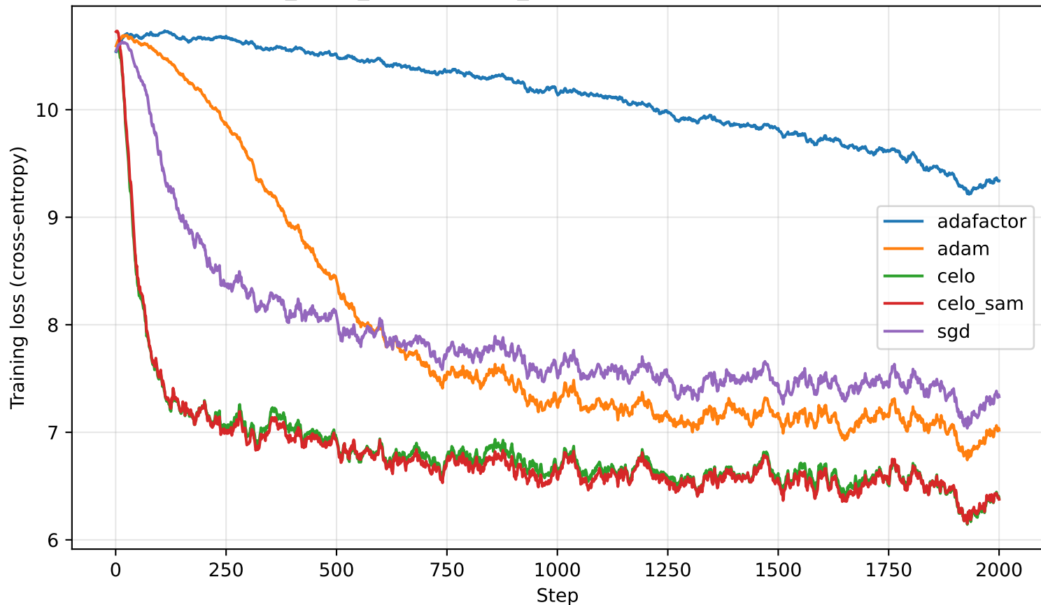
TransformerLM_LM1B_MultiRuntime_0: Training Loss vs Step (EWMA span=50)
