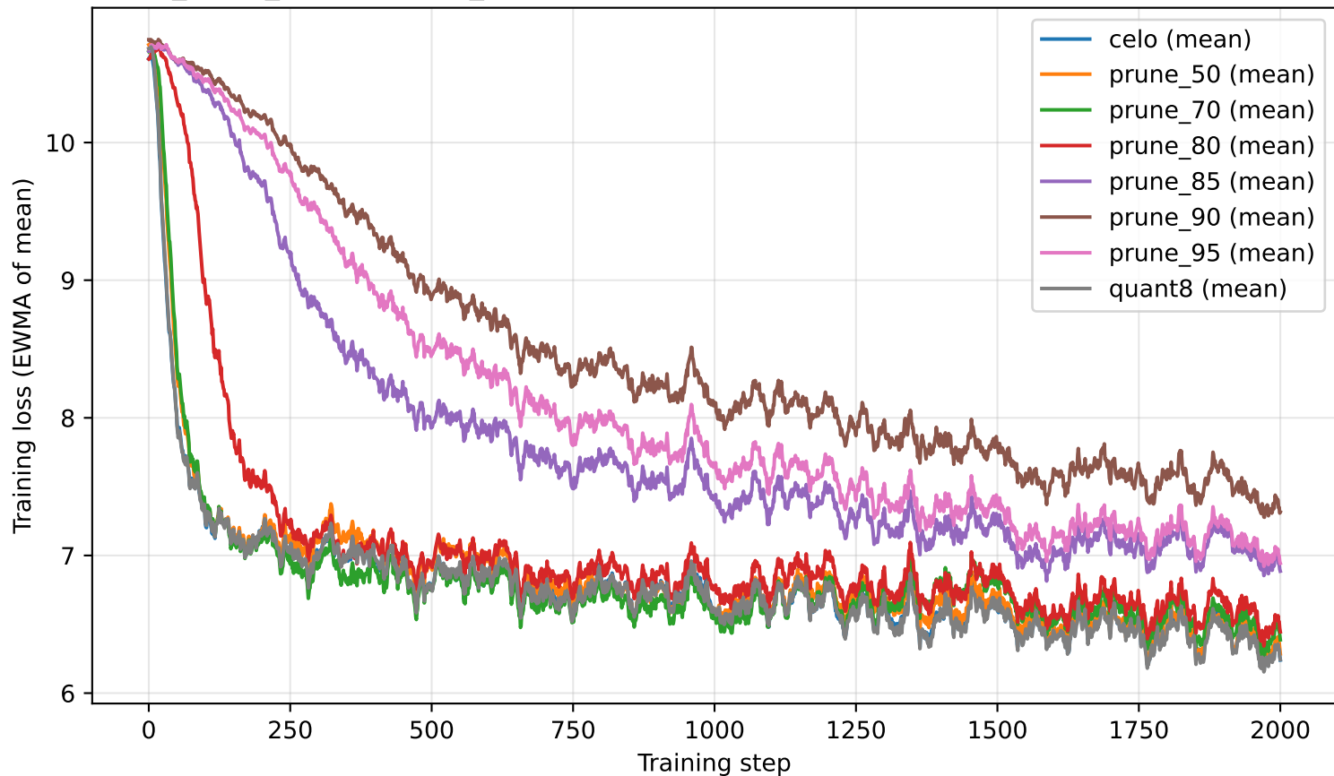
transformerLM_LM1B_MultiRuntime_0: CeLO compression sweep (mean \pm stderr over 1 seeds, sp
