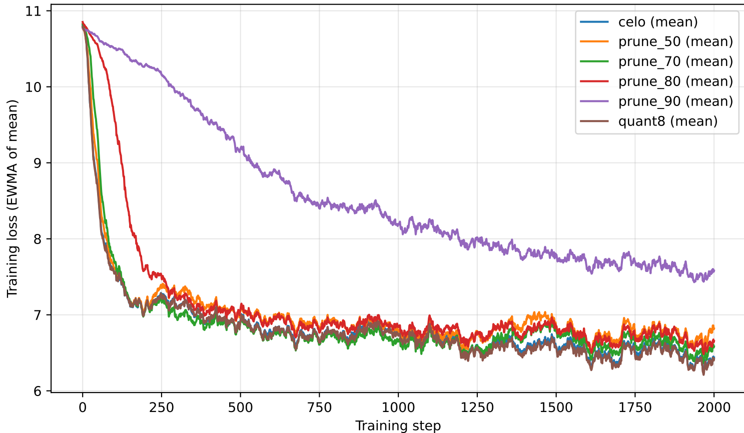
CeLO compression sweep: mean \pm stderr over 1 seeds (span=50)
