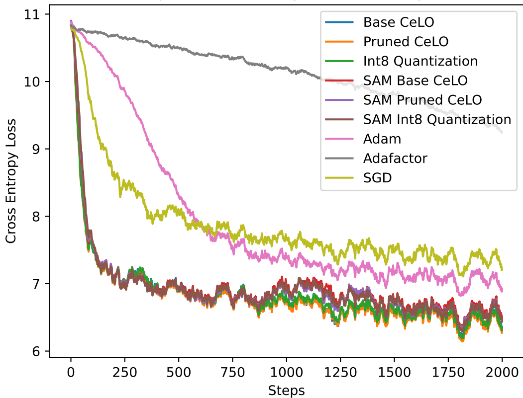
Optimizers Training Losses vs. Step
