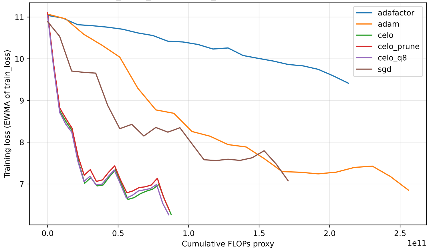
TransformerLM_LM1B_MultiRuntime_0: Training Loss vs FLOPs (EWMA span=5)
