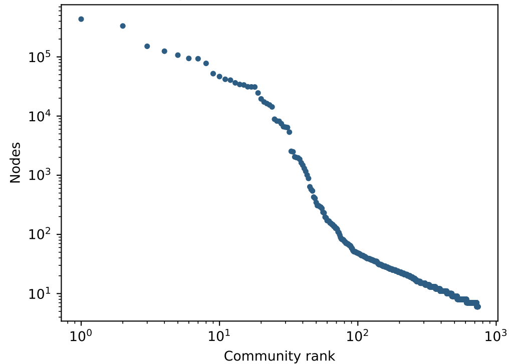
(a) Independent Leiden community sizes
