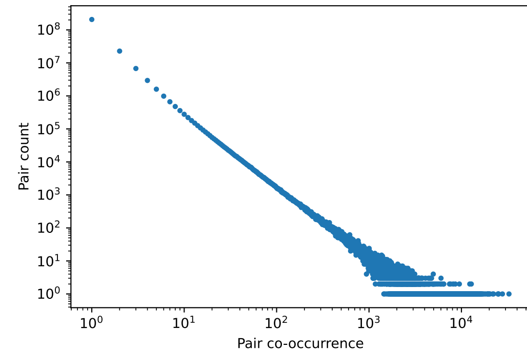
(c) Pair co-occurrence (local exact)
