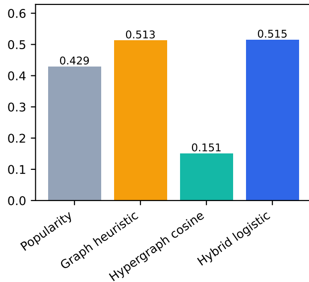
MRR
