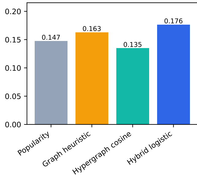
Micro Recall@100
