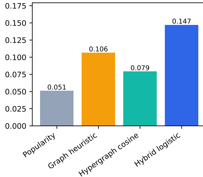
Micro Recall@50
