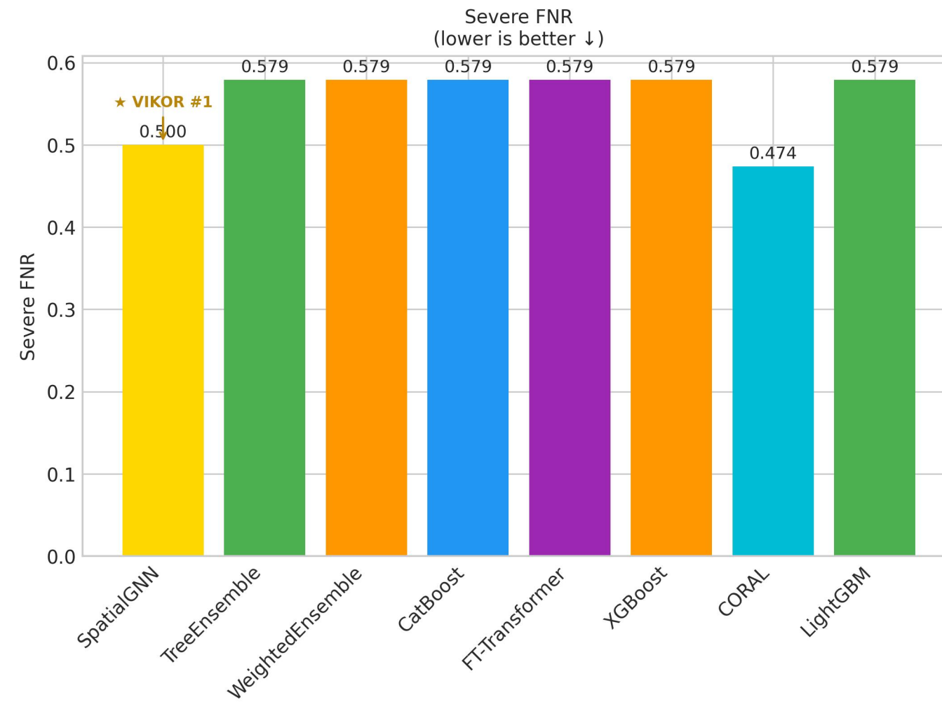
Model Performance Comparison (gold bar = VIKOR-selected best model)
