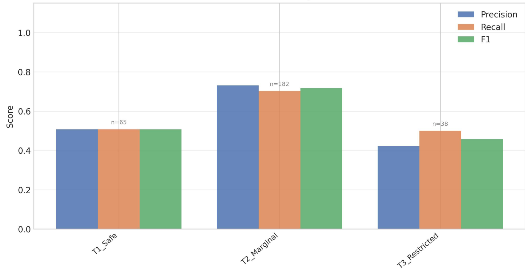
Per-Class Metrics — SpatialGNN
