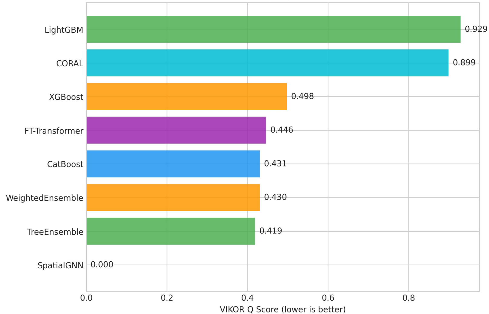
Model Rankings by VIKOR Q Score
