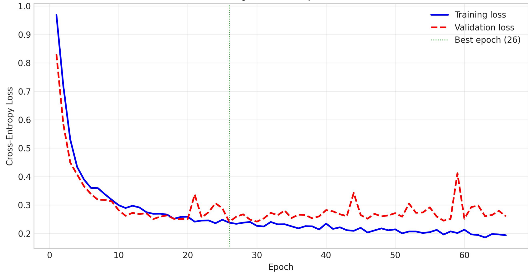
Learning Curves — SpatialGNN
