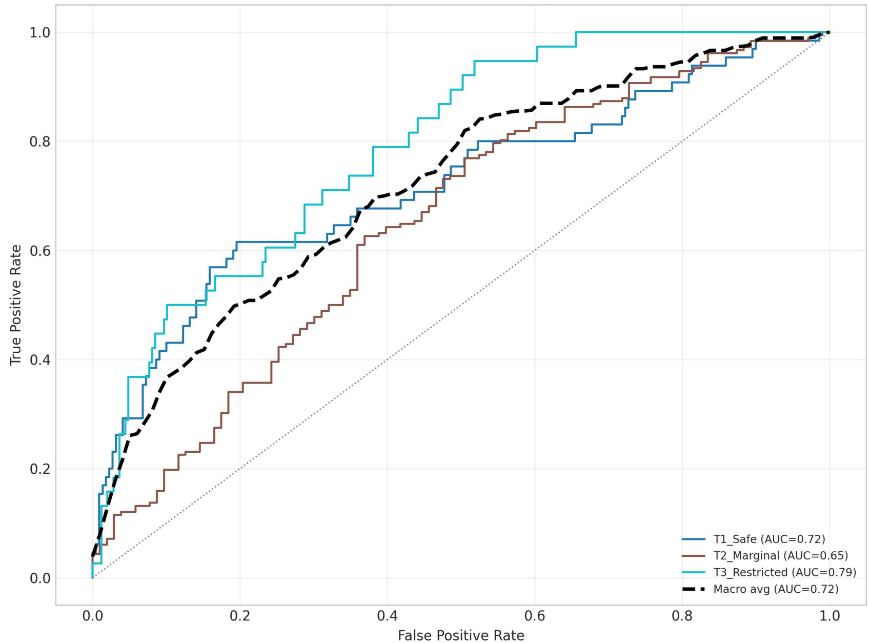
ROC Curves (One-vs-Rest) — SpatialGNN
