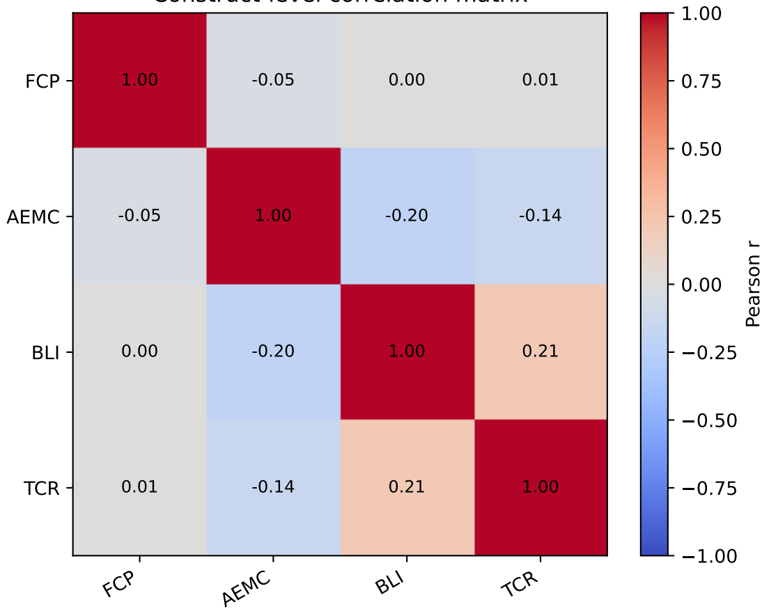
Construct-level correlation matrix
