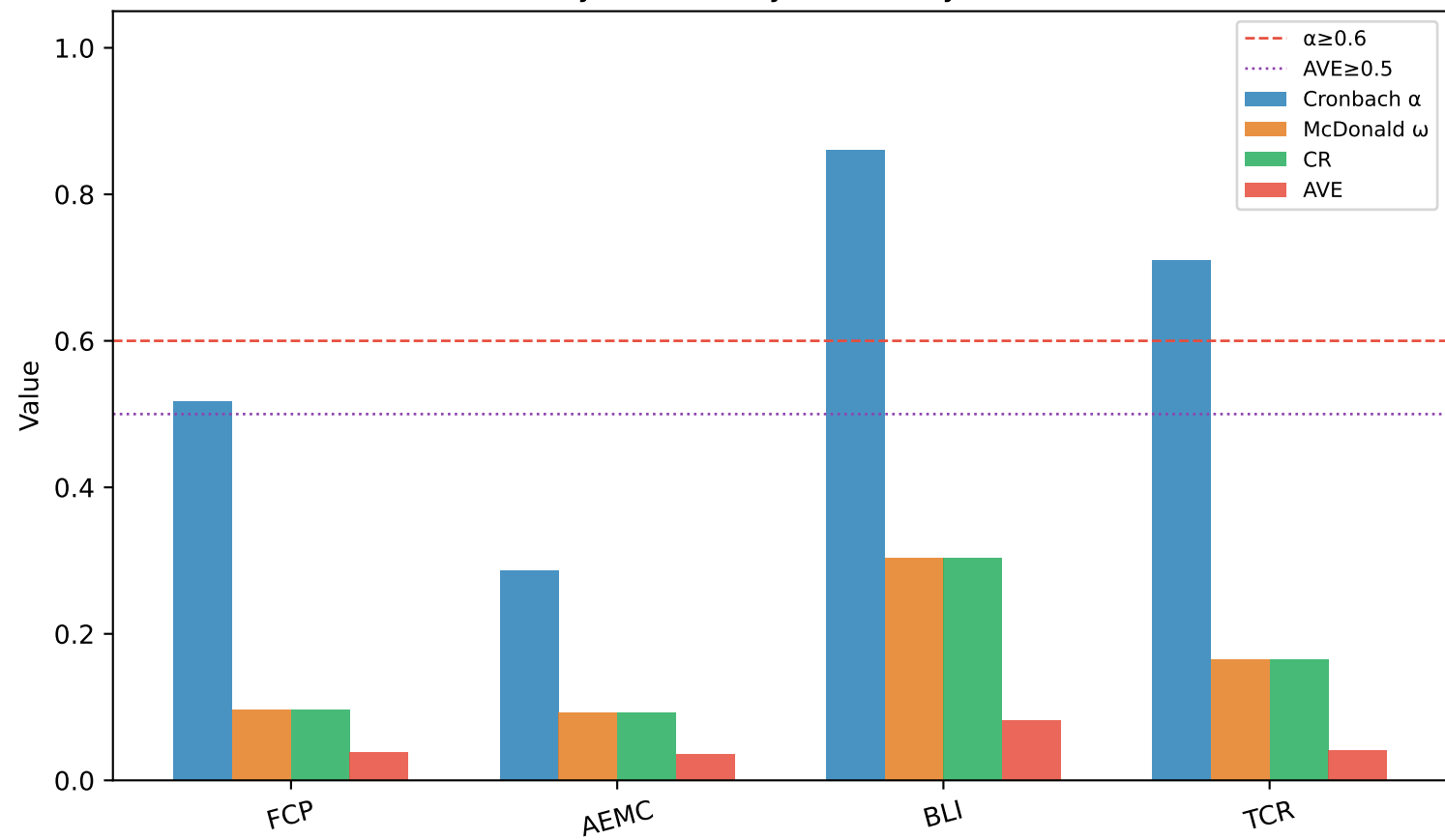
Reliability and validity metrics by construct
