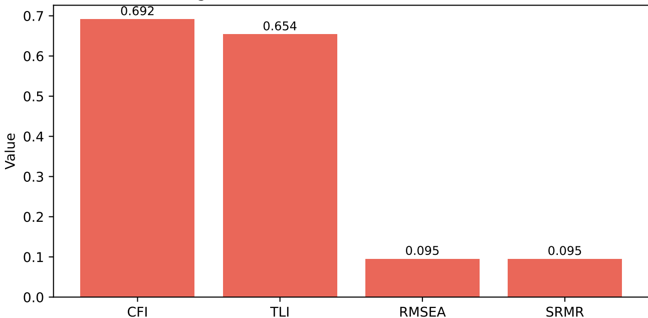
Route 2: CFA global fit indices (green = meets conventional threshold)
