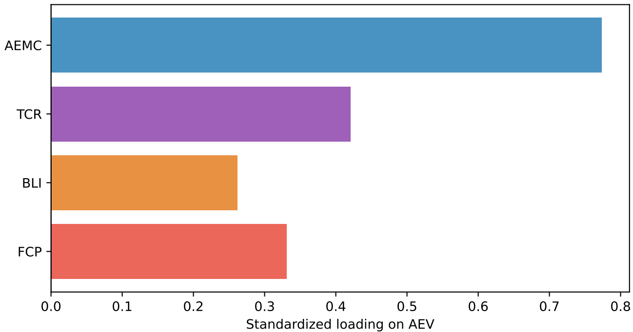
Route 2: second-order AEV structural loadings (Option 2A)
