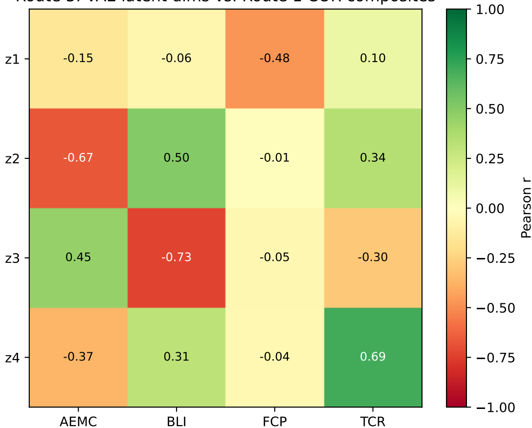
Route 3: VAE latent dims vs. Route 1 COR composites
